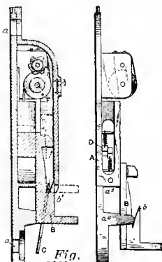
Fig. 3899a. BEASLEY'S SEAL LOCK.
